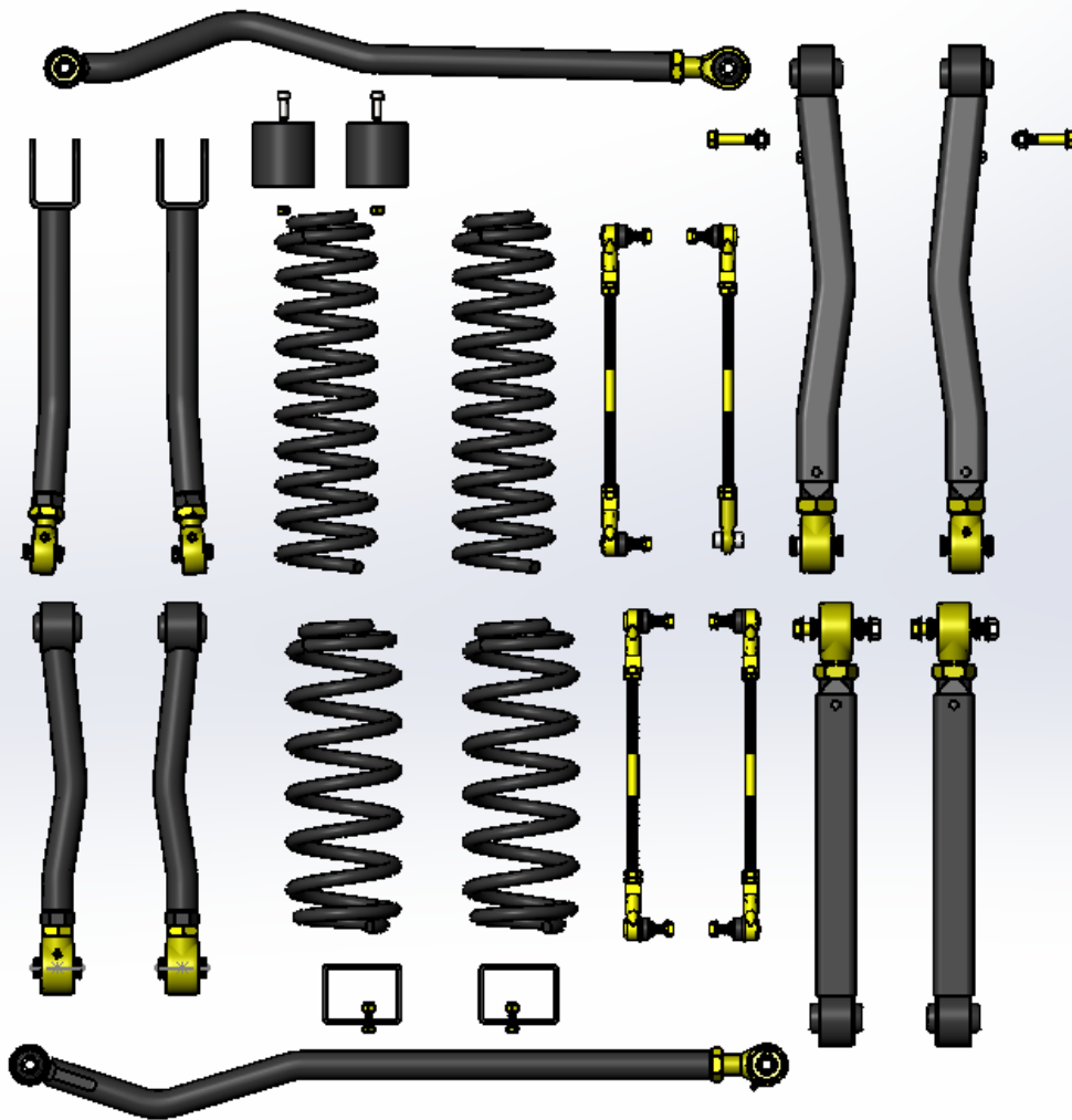
2909025 Jeep Wrangler 2.5" Premium Lift Kit (2018 & Up, JL)
